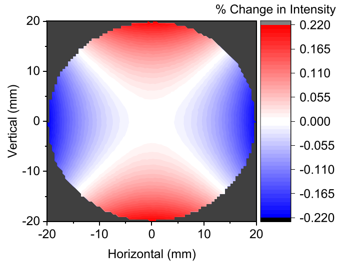
Figure 4. Percentage change in intensity of the beam over its cross-section at the beam-stop when the retarder rotates through 45^\circ .
