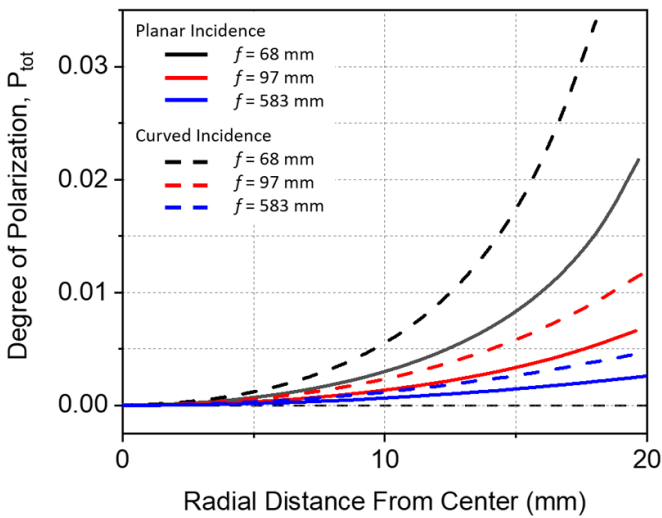
Figure 3. Degree of Fresnel-induced polarization, P_{tot} , as a function of distance from the center of the beam (i.e. along the black line in figure 2(d)) for focal lengths f = 68 mm (black), f = 97 mm (red), and f = 583 mm (blue). The curves for the 583-mm focal length have been multiplied by a factor of 20. The solid lines correspond to the planar side of the lens facing upstream, while the dashed lines are for the curved side facing upstream.
