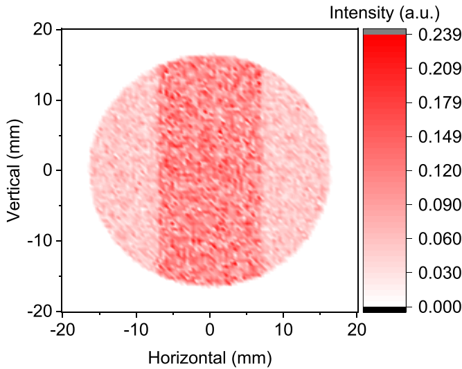
Figure 6. A map of intensity incident upon the collection lens for the simulated, fully linearly-polarized Ne 640-nm p \rightarrow s fluorescence. The difference in intensity between the sides and the middle portions of the beam has been exaggerated for the sake of clarity.
